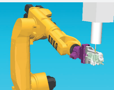
Deburring. The Workpiece can be mounted directly on the Robot Arm
